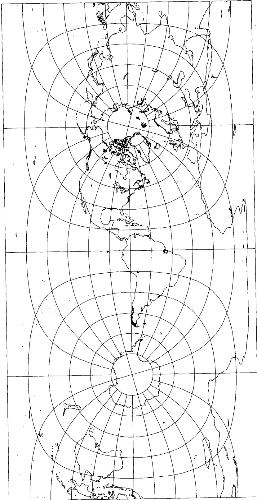
FIGURE 19.—Cassini projection. A transverse Equidistant Cylindrical projection used for large-scale mapping in France, England, and several other countries. Largely replaced by conformal mapping.
