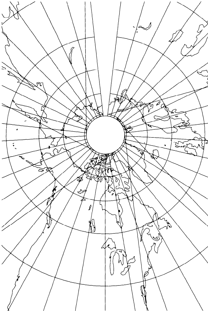
FIGURE 51.—Conic Satellite-Tracking projection (standard parallel 80.9° N.). Landsat 1, 2, 3 orbits. Groundtracks are as described on Fig. 50. The nearest approach to an azimuthal projection for these orbits. Inner circle is tracking limit and circle of tangency.
