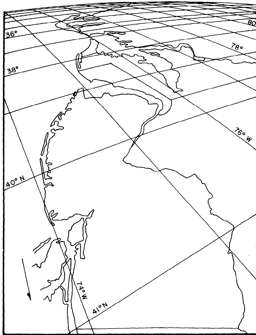
FIGURE 37.—Tilted Perspective projection. Eastern seaboard viewed from a point about 160 km above Newburgh, N. Y. Parameters using symbols in text: \phi_1 = 41^\circ 30' \text{ N. lat.} , \lambda_0 = 74^\circ 00' \text{ W. long.} , \omega = 55^\circ , \gamma = 210^\circ , P = 1.025 . 1^\circ graticule.
