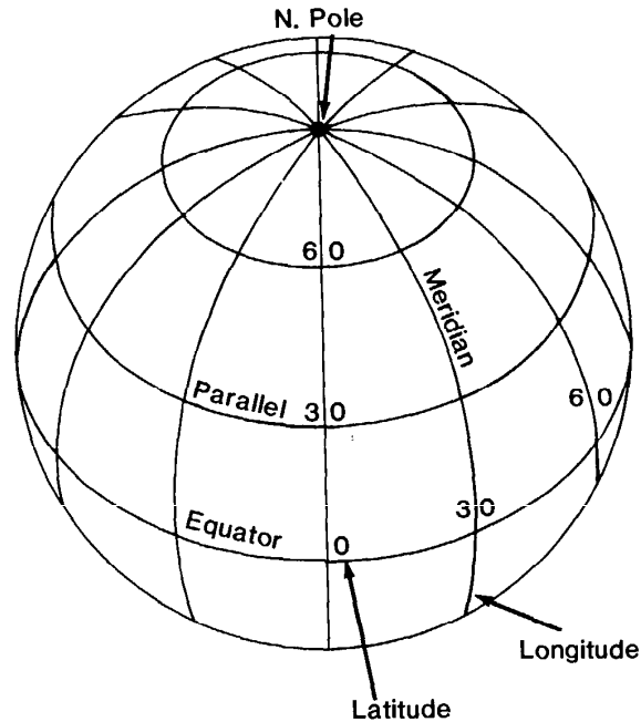
FIGURE 2.—Meridians and parallels on the sphere.
