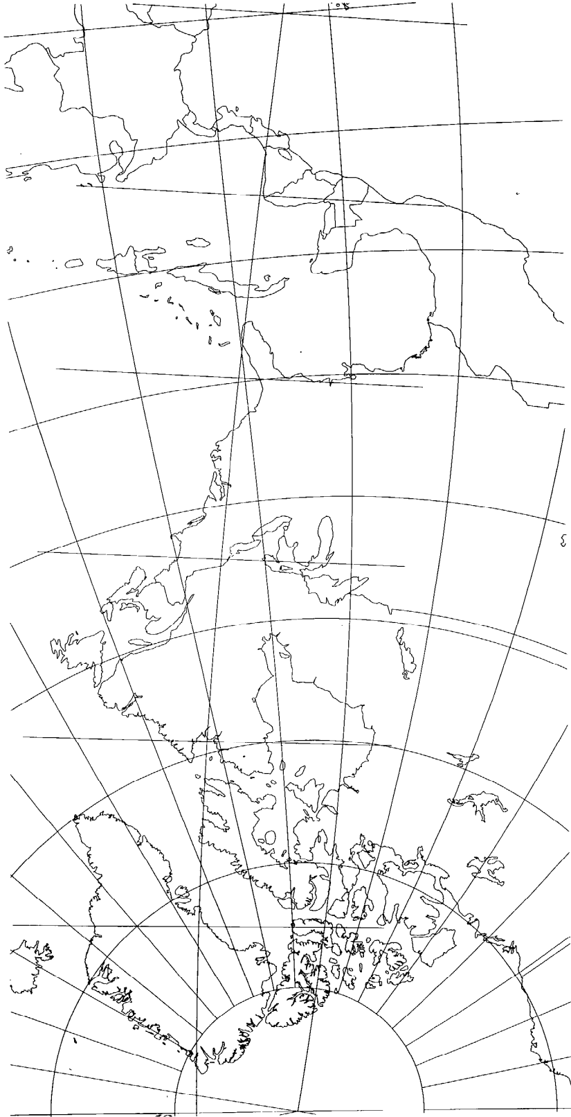
FIGURE 47.—One quadrant of the Space Oblique Mercator projection for Landsat 5, path 15. An “enlargement” of part of figure 46 beginning at the North Pole.
