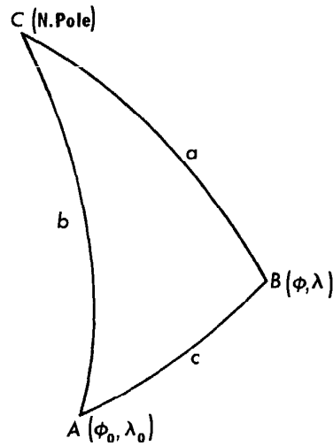
FIGURE 5.—Spherical triangle.
