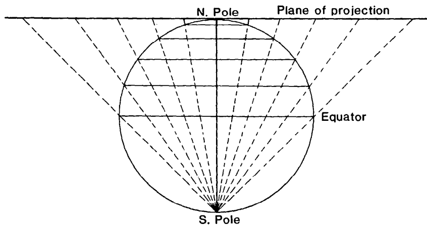
FIGURE 31.—Geometric projection of the polar Stereographic projection.
